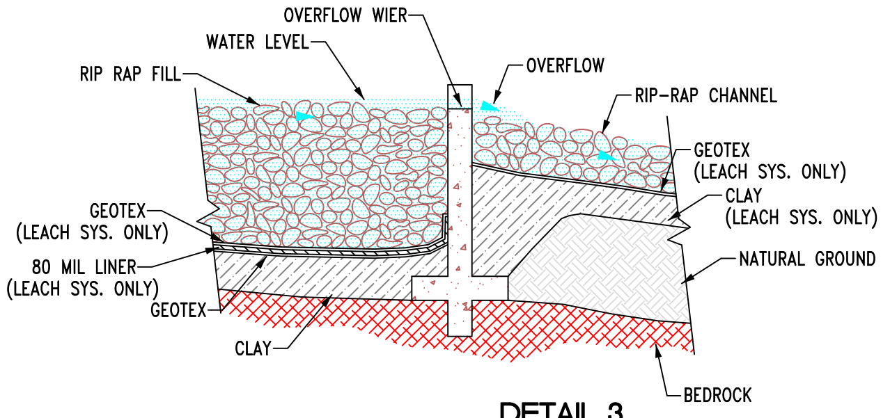
DETAIL 3 CROSS SECTION AT OVERFLOW WIER FOR FLOWS IN EXCESS OF 10YR 24HR EVENT
